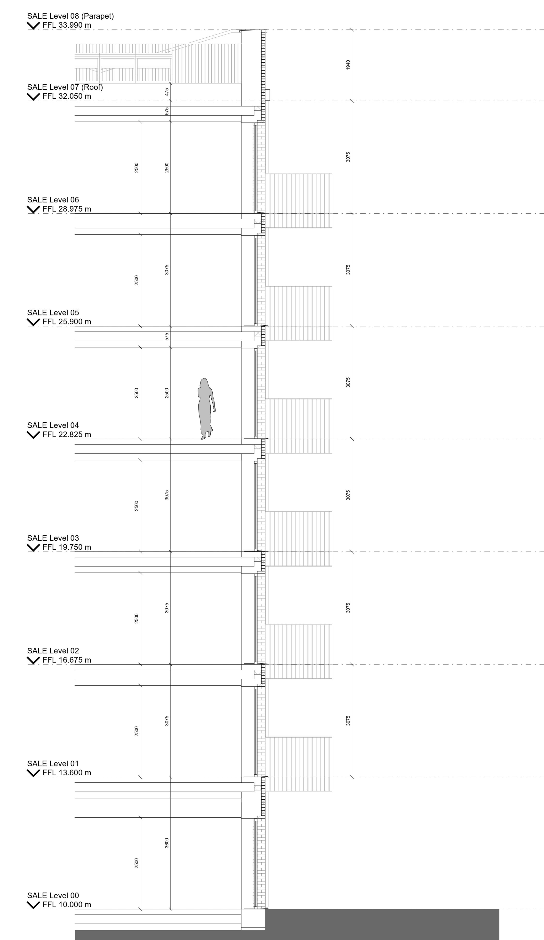
2 SALESIANS BLOCK A - Bay Study 01 Section 1 : 50
