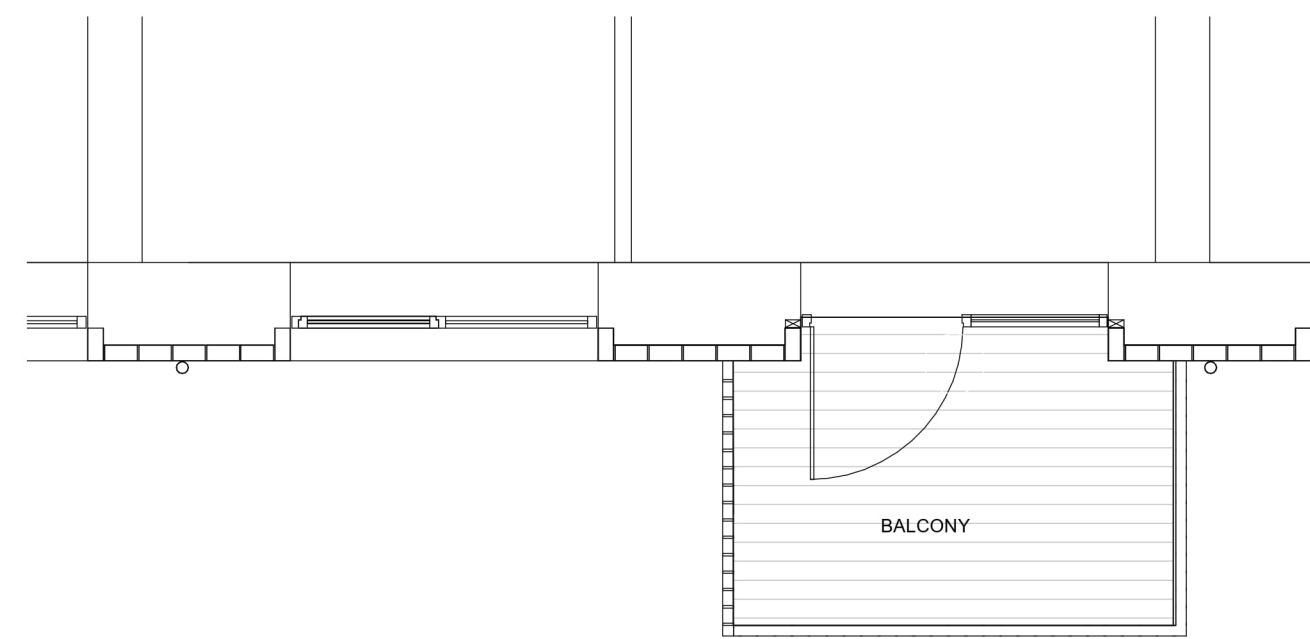
3 SALESIANS BLOCK A - Bay Study 01 Plan Detail 1 : 50
